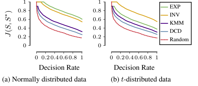
Figure 3: [Higher is better.] Decision rate plots of the Jaccard similarity between recovered and true set of variables affected by selection bias. Left: Experiments on Gaussian distributed data. EXP outperforms INV slightly, and both outperform KMM and DCD significantly. Right: Experiments on t -distributed data. INV outperforms EXP, which in turn outperforms KMM and DCD significantly. In both cases, all methods significantly outperform random guessing.
