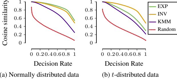
Figure 2: [Higher is better.] Decision rate plots of the cosine similarity between discovered and true selection boundary. Left: Experiments on Gaussian distributed data. EXP outperforms INV slightly, and both outperform KMM significantly. Right: Experiments on t -distributed data. INV outperforms both EXP and KMM significantly. In both cases, all methods significantly outperform random guessing.
